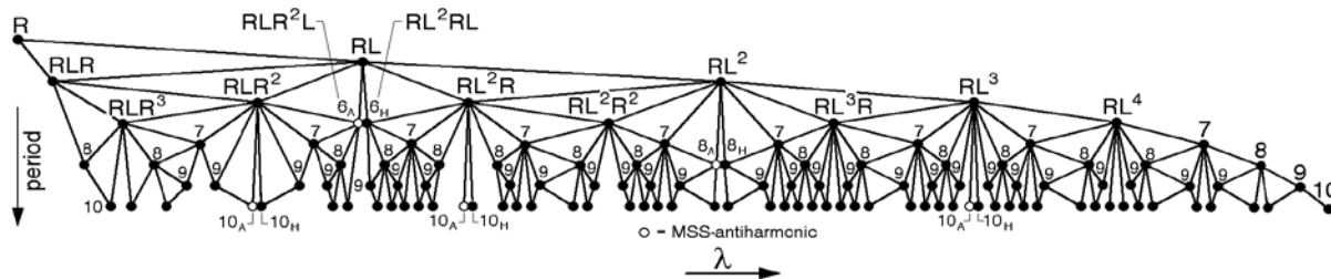
Figure 2. A sketch of the successive application of the Metropolis, Stein, and Stein theorem in the logistic map x_{n+1} = \lambda x_n(1-x_n) for p \leq 10 . Symbolic sequences for periods p \leq 6 are shown.
