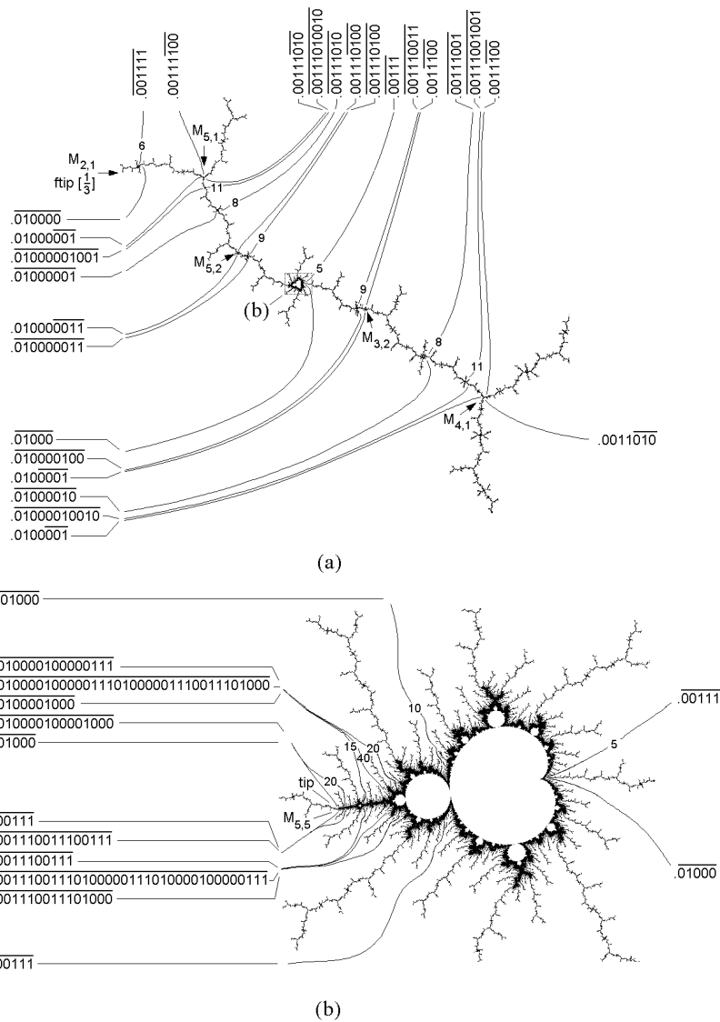
Figure 6. (a) Magnification of the branch 11 of the shrub (1/3) shown in Figures 5 (b) and (c), where the period-5 representative can be better observed. (b) Magnification of such a period-5 representative shown in the rectangle b marked in (a), with some of its important external arguments.
